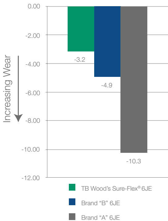
Figure 6: Wear test results; 6JE TB Wood’s Sure-Flex Plus coupling vs. competition
