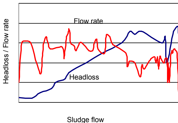
Headloss and flow rate vrs sludge flow
